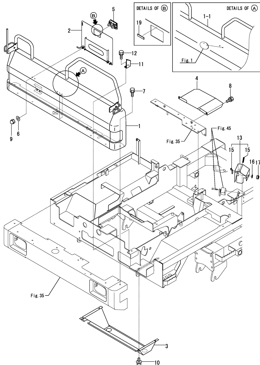
Fig.36. COVER
