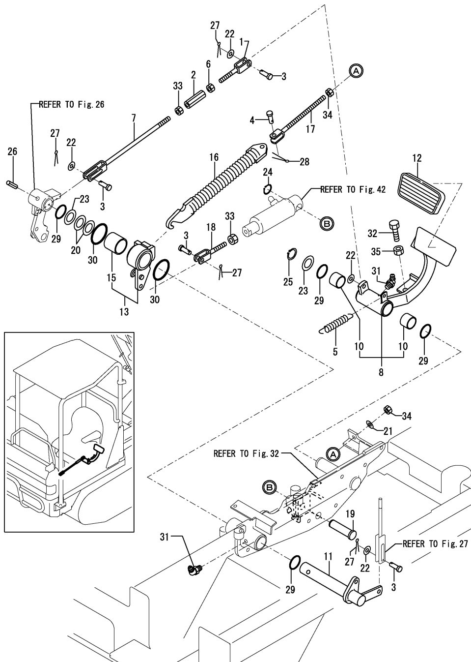
Fig.28. BRAKE(PEDAL & ROD)(REAR)
