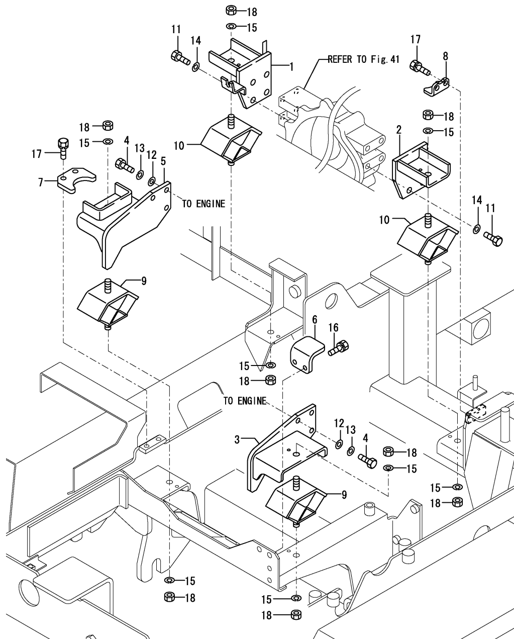
Fig.8. ENGINE MOUNT
