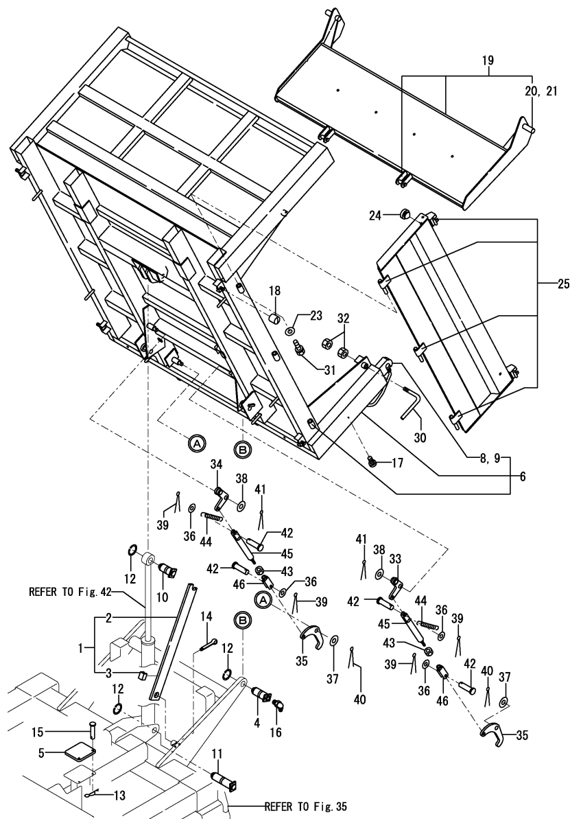
Fig.50. WAGON
