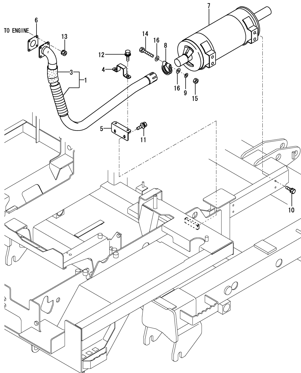
Fig.5. EXHAUST PIPE
