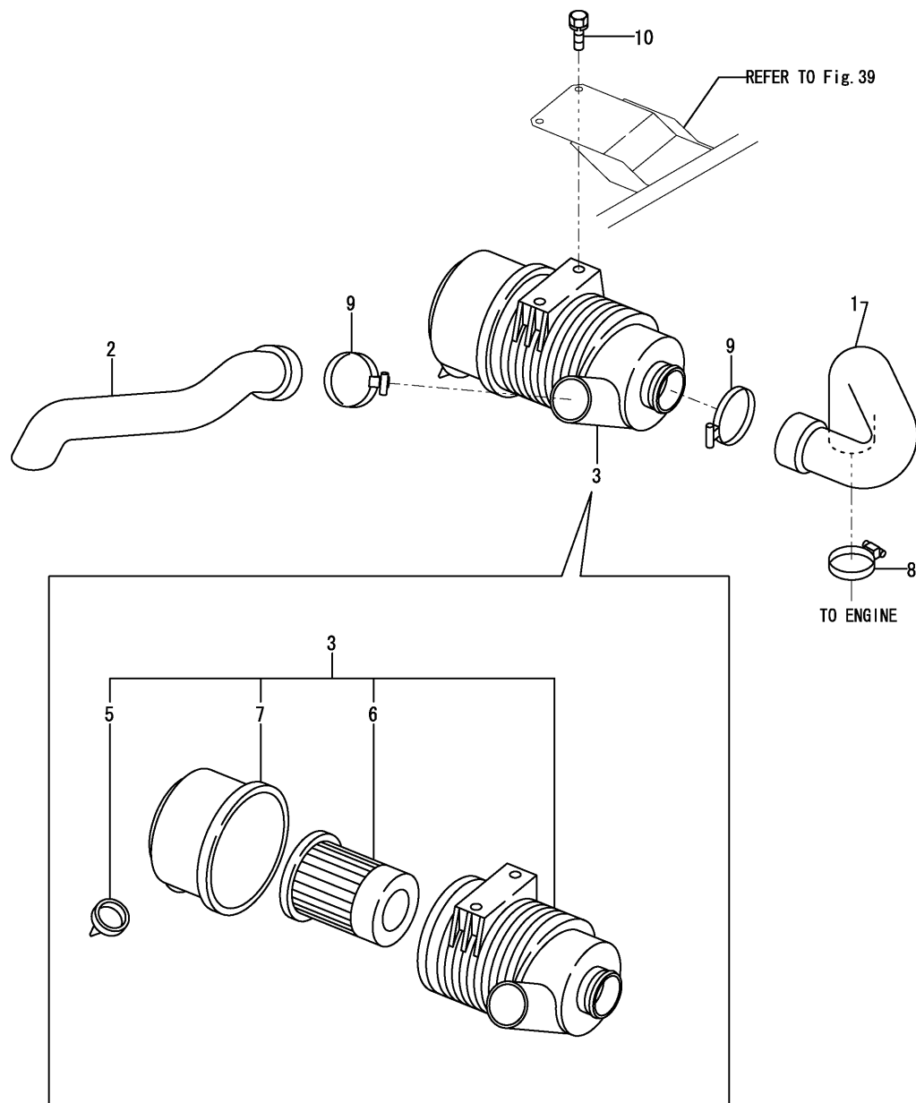
Fig.6. SUCTION PIPE
