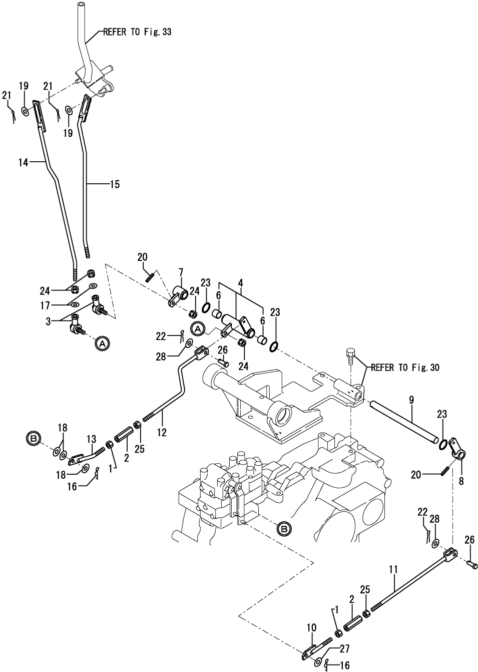
Fig.34. STEERING LINK
