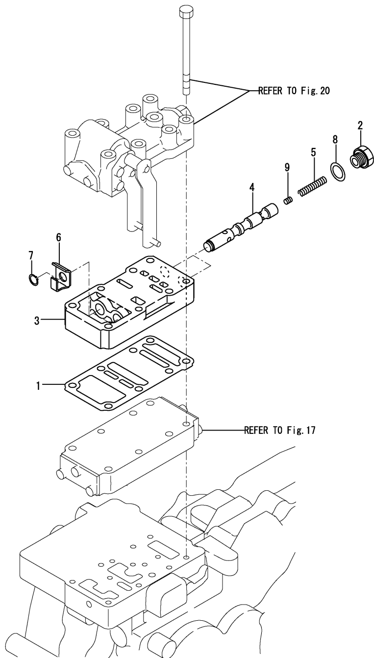
Fig.18. SB VALVE
