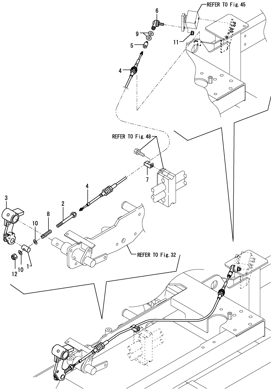
Fig.26. INCHING LINK
