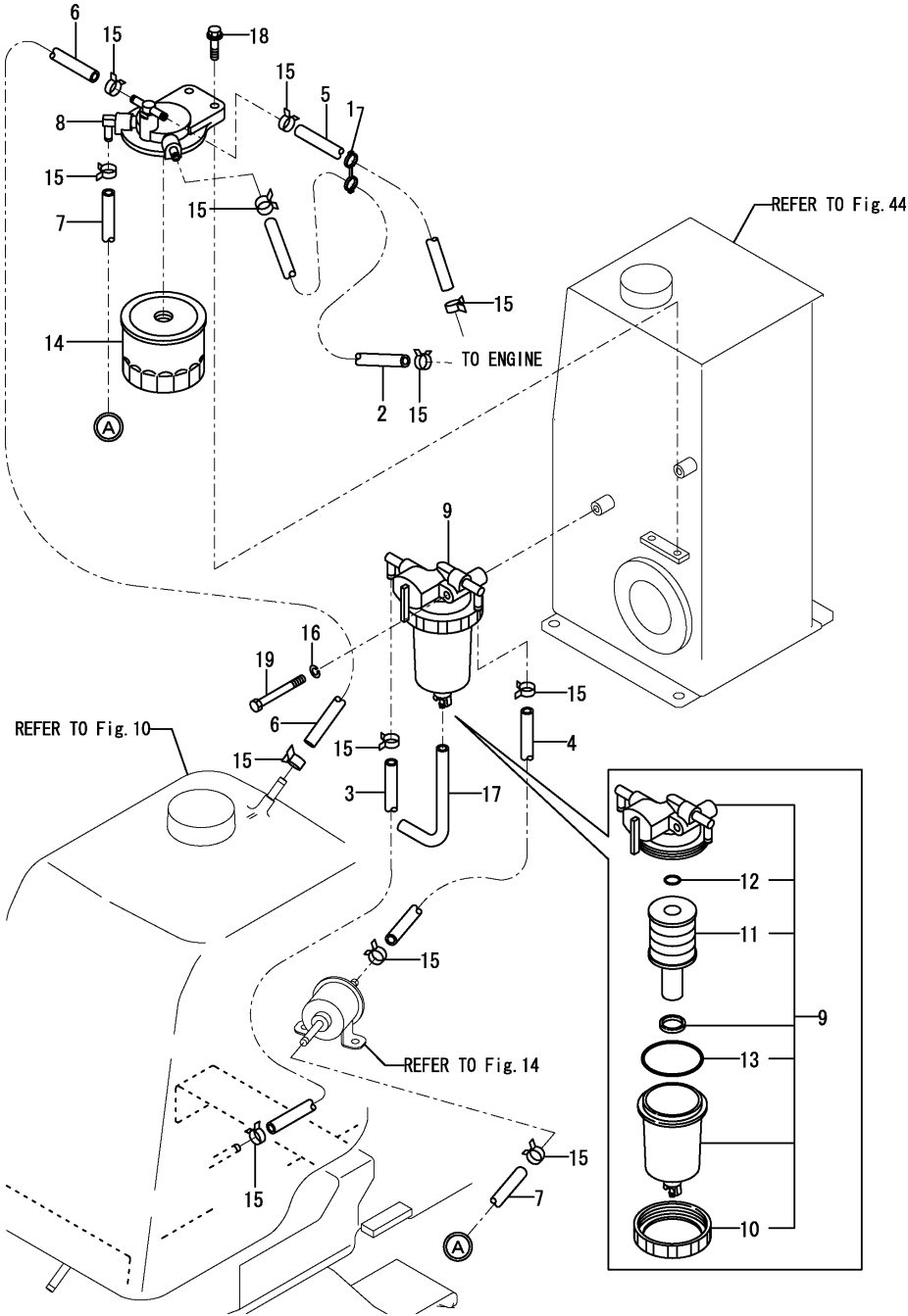
Fig.11. FUEL PIPE
