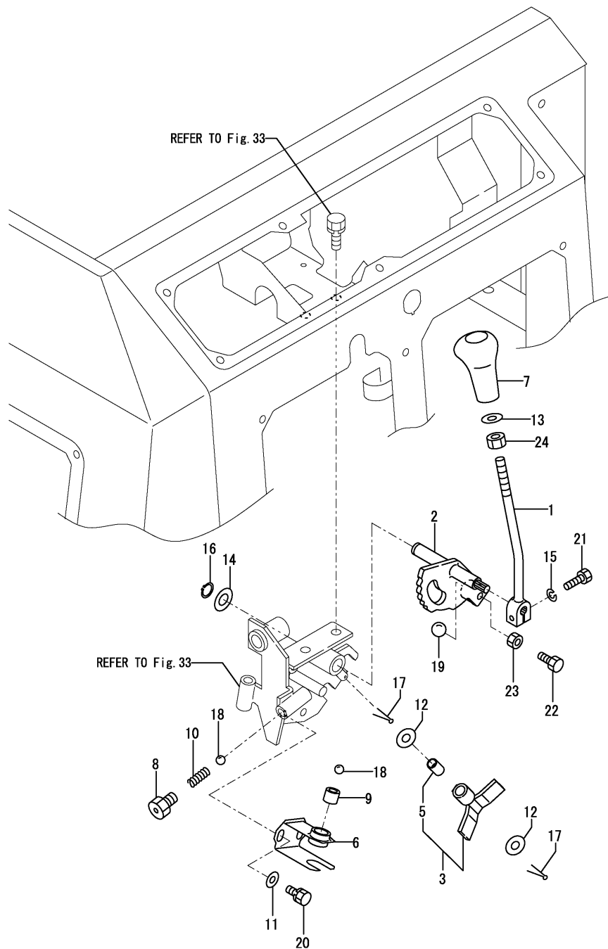
Fig.25. FR LEVER
