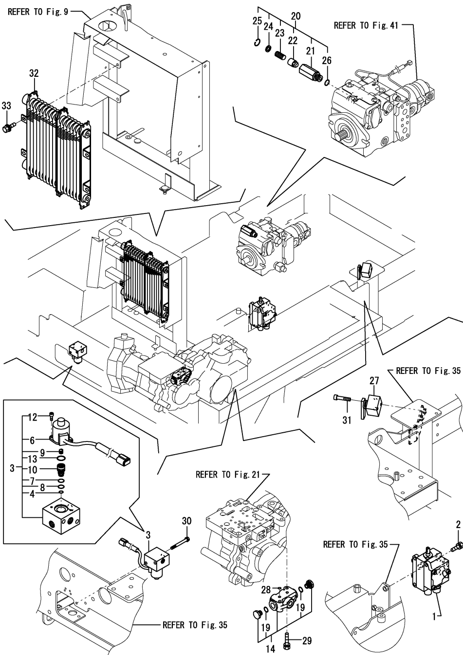
OCS10-M52500 VEHICLE C30RUS-2B Fig.45. HYD.OIL VALVE & LUB.OIL COOLER
