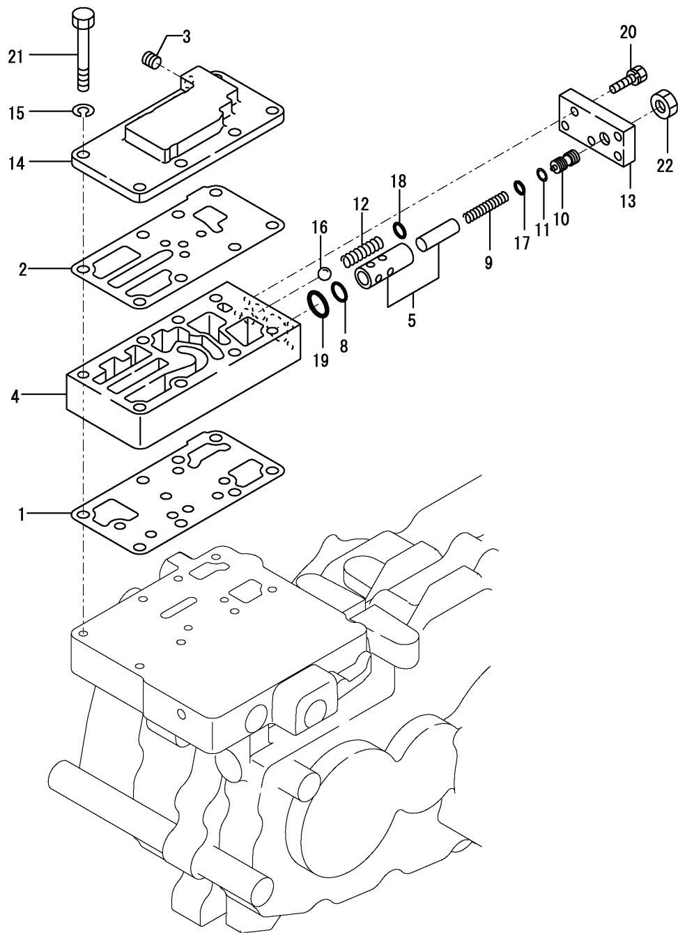
Fig.16. RELIEF VALVE
