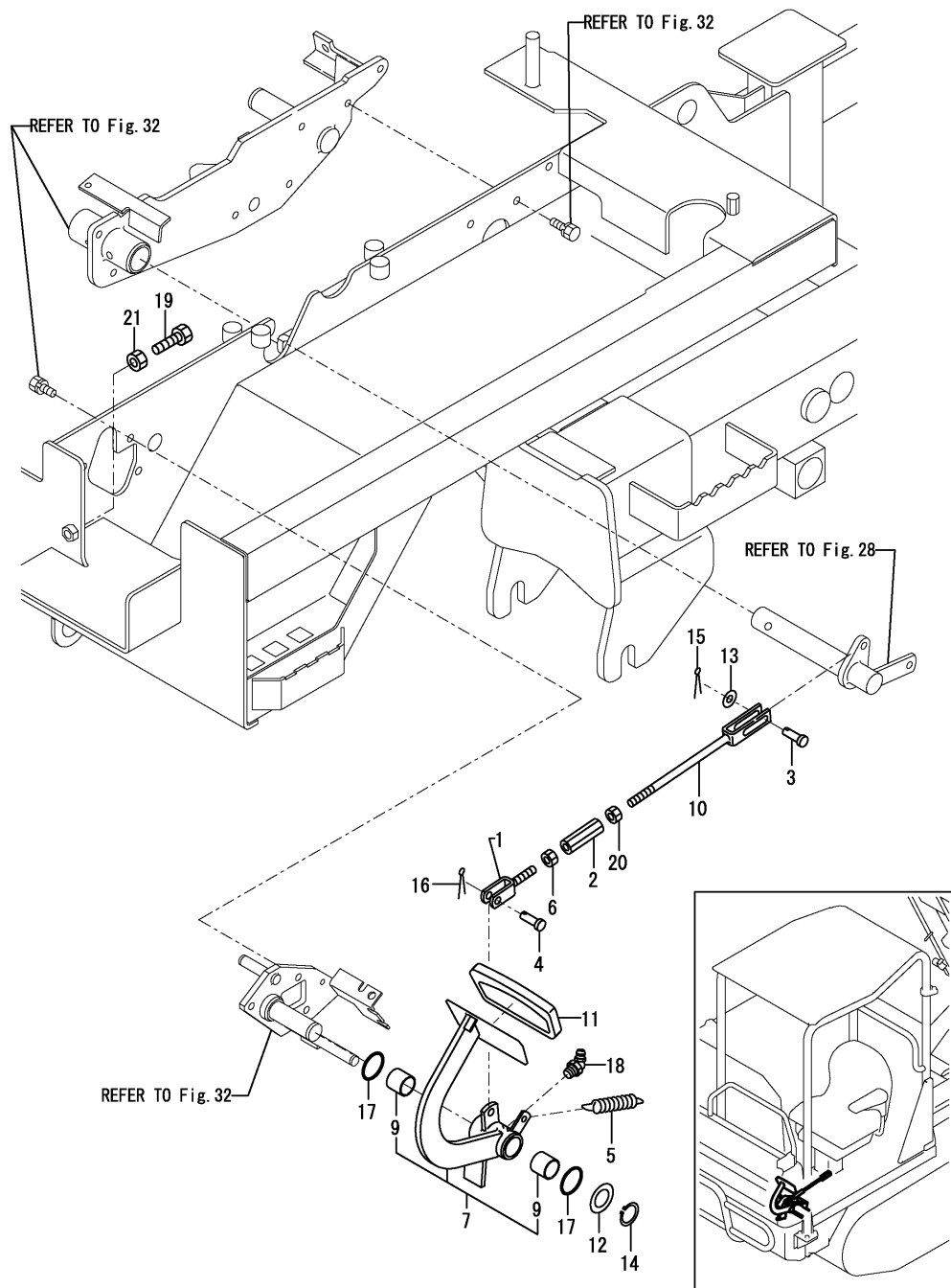
Fig.29. BRAKE(PEDAL & ROD)(FRONT)
