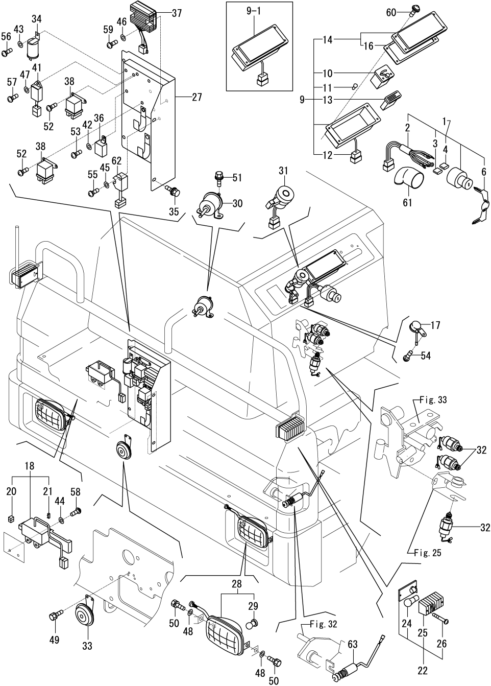
OCS10-M52500 VEHICLE C30RUS-2B Fig.14. ELECTRIC PART(EQUIPMENT)
