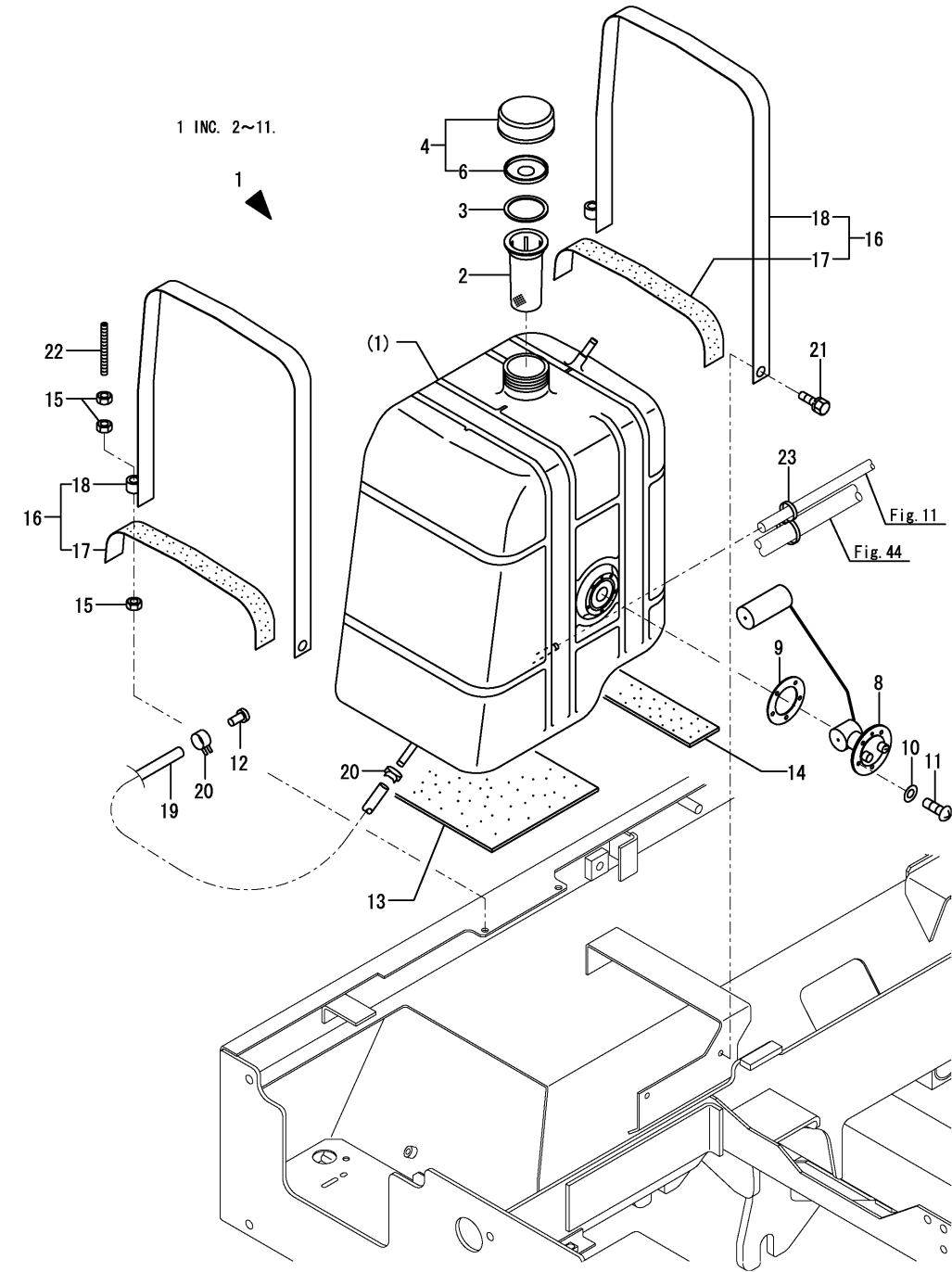
Fig.10. FUEL TANK
