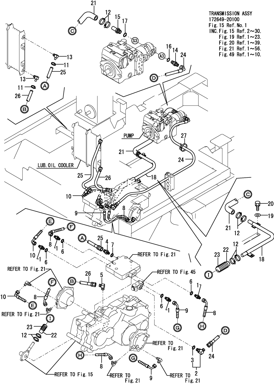
OCS10-M52500 VEHICLE C30RUS-2B Fig.49. HYD.OIL PIPING(REDUCTION)
